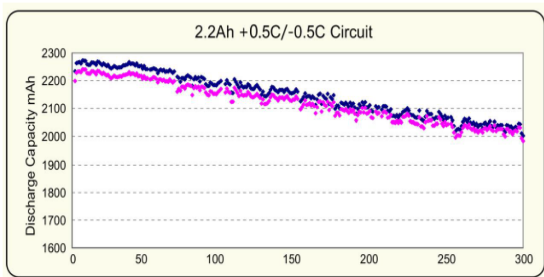
Discharge Capacity vs Cycle Life Graph for 2 Sample Batteries
