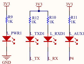
Indicator light
