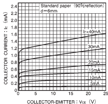
Fig.5 Output characteristics
