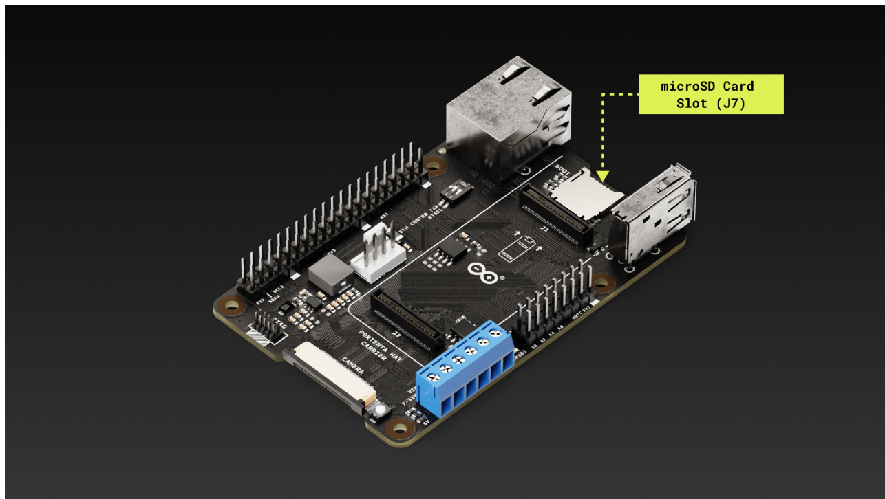
Figure 10. microSD card slot of the Portenta Hat Carrier
