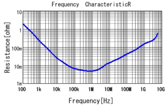
■ GRM155R60J106ME15 R DCOV, 25degC
