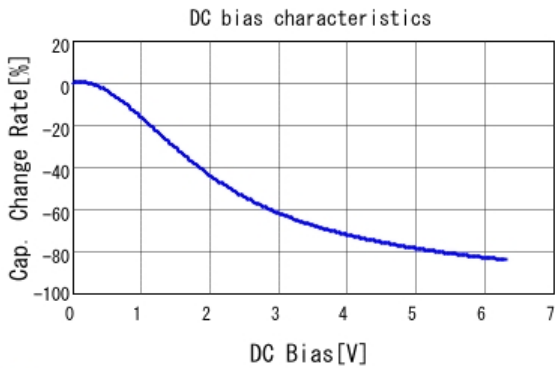
■ GRM155R60J106ME15 C-DC bias capchange, 25.0degC, ACO.
