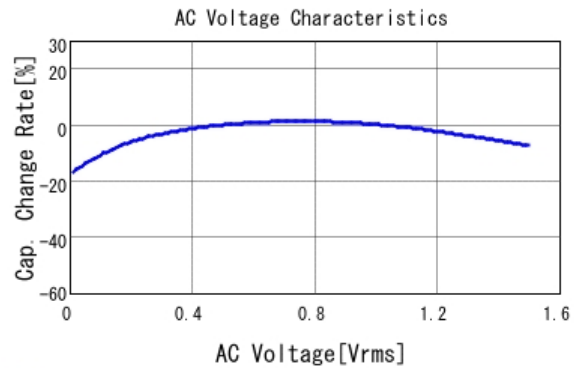
■ GRM155R60J106ME15 C-AC Voltage capchange, DCOV, 25.0d
