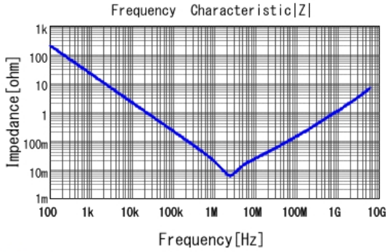
■ GRM155R60J106ME15 |Z| DCOV, 25degC
