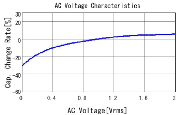
■ GRM155C81E105KE11 C-AC Voltage capchange, DCOV, 25.0d
