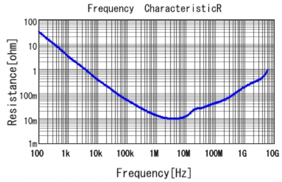
■ GRM155C81E105KE11 R DCOV, 25degC
