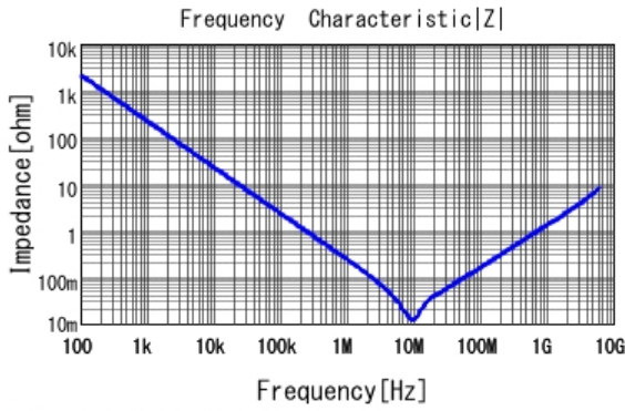
■ GRM155C81E105KE11 |Z| DCOV, 25degC
