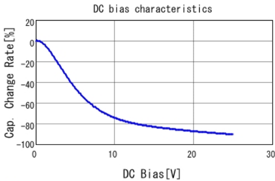
■ GRM155C81E105KE11 C-DC bias capchange, 25.0degC, AC1V
