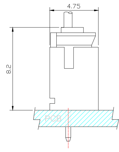
ASSEMBLY LAYOUT
