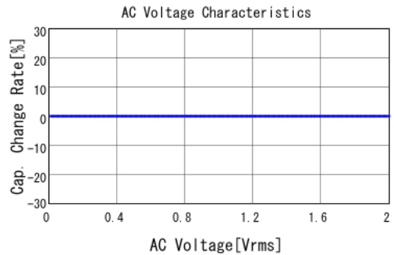
■ GRM1885C1H472JA01 C-AC Voltage capchange, DCOV, 25.0d
