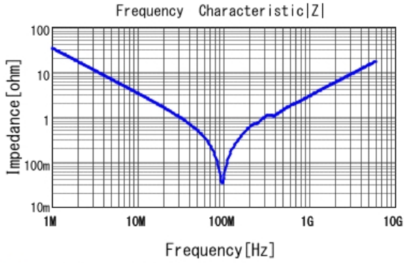
■ GRM1885C1H472JA01 |Z| DCOV, 25degC
