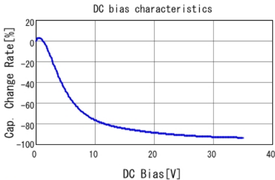
■ GRM188R6YA225KA12 C-DC bias capchange, 25.0degC, AC1.
