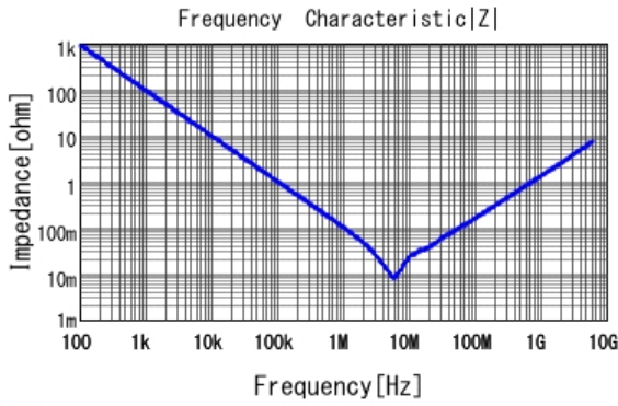
■ GRT155R61E225KE13 |Z| DCOV, 25degC
