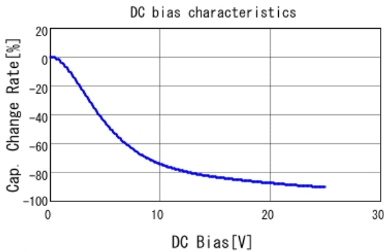
■ GRT155R61E225KE13 C-DC bias capchange, 25.0degC, AC1V
