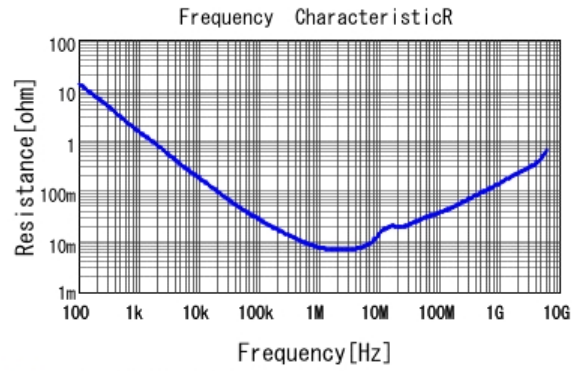
■ GRT155R61E225KE13 R DCOV, 25degC
