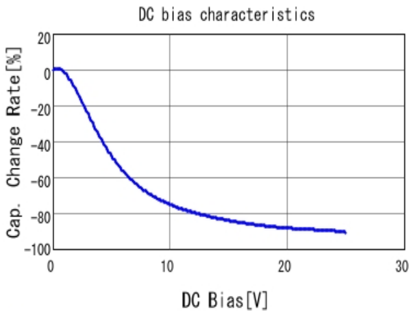
■ GRT188R61E475KE13 C-DC bias capchange, 25.0degC, AC1V
