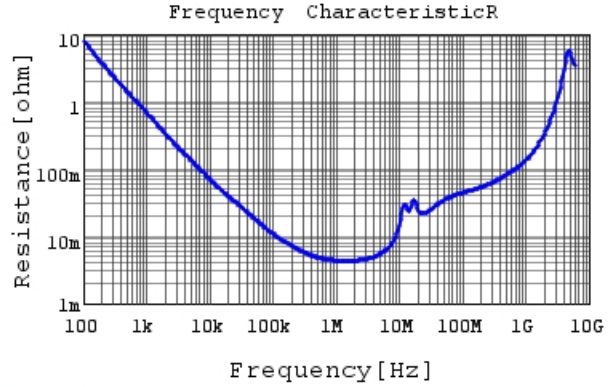
GCM21BR71H105KA03 R DCOV, 25degC
