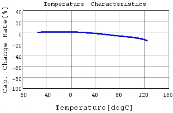
GCM21BR71H105KA03 C-Temp. capchange, DC0.0V,
