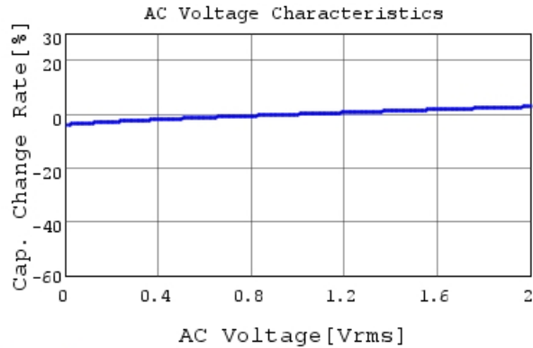
GCM21BR71H105KA03 C-AC Voltage capchange, DC
