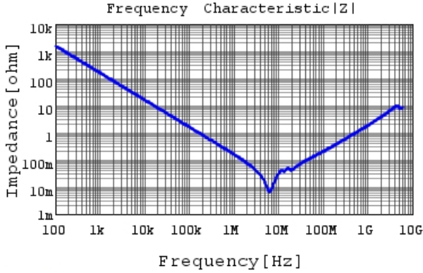
GCM21BR71H105KA03 |Z| DCOV, 25degC
