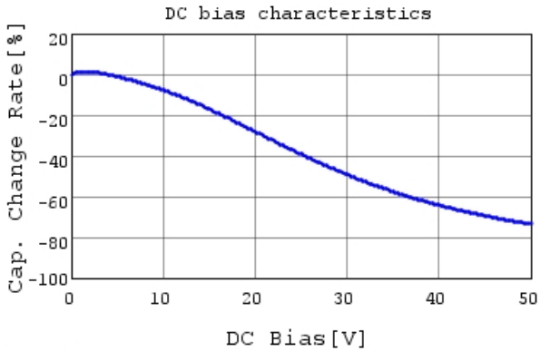
GCM21BR71H105KA03 C-DC bias capchange, 25.0c
