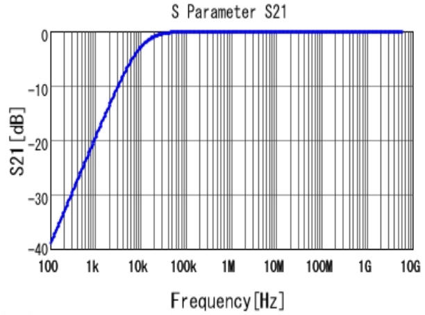
■ GRM033R61C224KE14 S21 DCOV, 25degC
