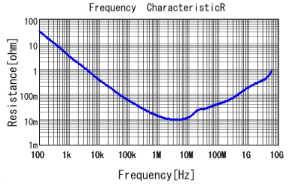
■ GRM155R6YA105ME11 R DCOV, 25degC
