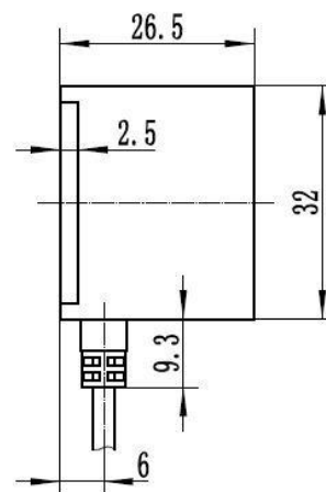
Figure 2. Top view of HPS-167C
