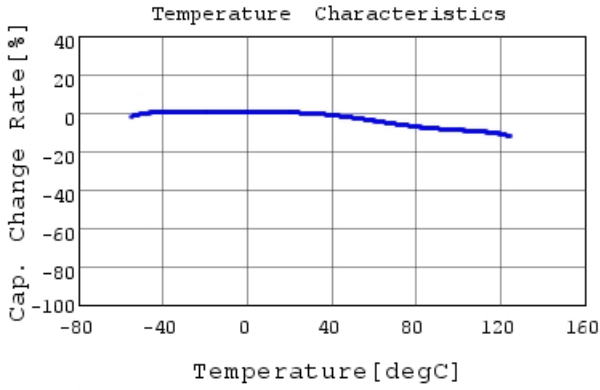
GCM31CR71H225KA55 C-Temp. capchange, DC0.0V,
