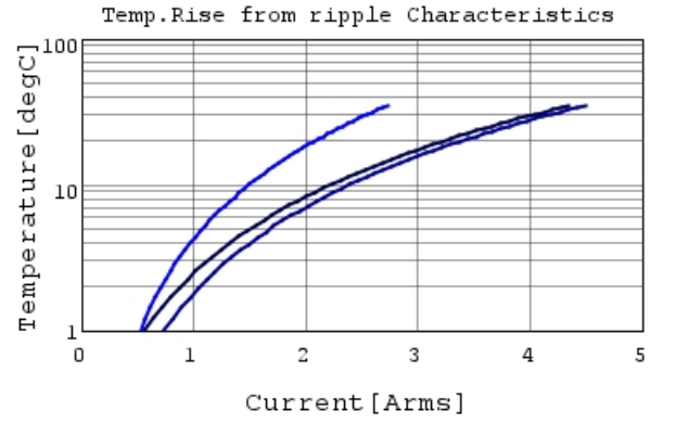
GCM31CR71H225KA55 Temp.rise — 100kHz
