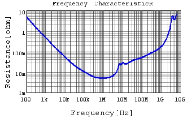
GCM31CR71H225KA55 R DC0V, 25degC
