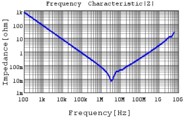
GCM31CR71H225KA55 |Z| DC0V, 25degC
