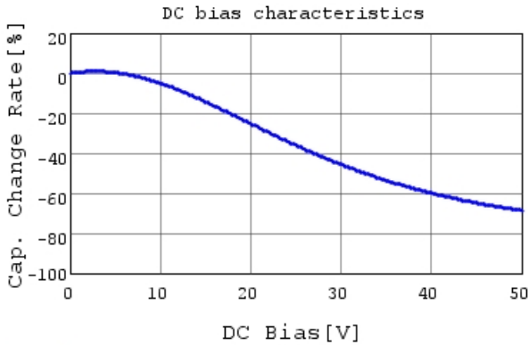
GCM31CR71H225KA55 C-DC bias capchange, 25.0c
