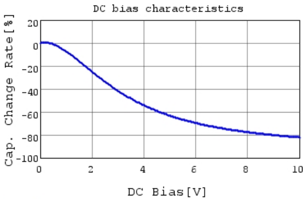
GRM21BR61A226ME51 C-DC bias capchange, 25.0c
