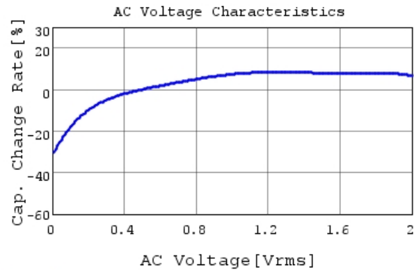
GRM21BR61A226ME51 C-AC Voltage capchange, DC
