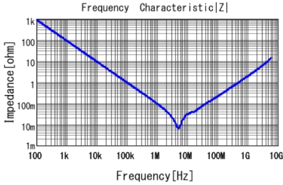
■ GRT188R61H225KE13 |Z| DCOV, 25degC
