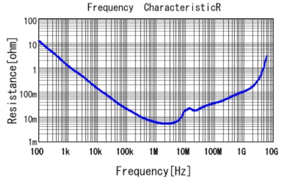
■ GRT188R61H225KE13 R DCOV, 25degC
