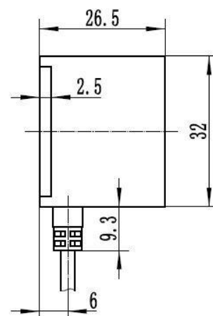
Figure 2. Side view of HPS-166U-L
