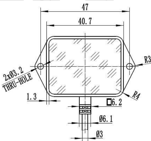
Figure 1. Front view of HPS-166U-L
