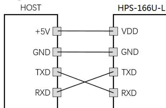
Figure. 3 Application schematic of the HPS-166U-L
