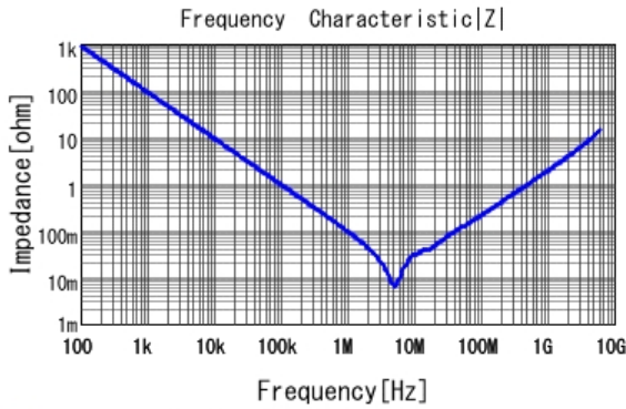
■ GRM188R61H225ME11 |Z| DCOV, 25degC
