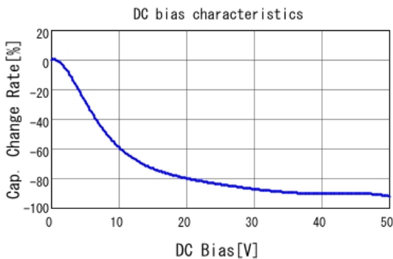
■ GRM188R61H225ME11 C-DC bias capchange, 25.0degC, AC1V
