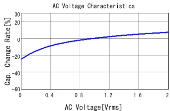
■ GRM188R61H225ME11 C-AC Voltage capchange, DCOV, 25.0d
