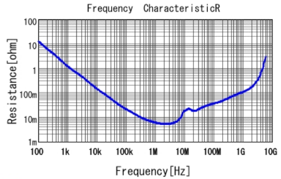
■ GRM188R61H225ME11 R DCOV, 25degC
