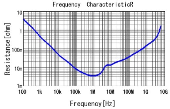
■ GRT188R61E106ME13 R DCOV, 25degC
