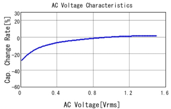
■ GRT188R61E106ME13 C-AC Voltage capchange, DCOV, 25.0d
