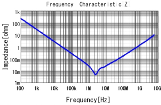
■ GRT188R61E106ME13 |Z| DCOV, 25degC
