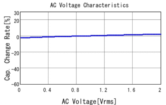
■ GRM188R72A104KA35 C-AC Voltage capchange, DCOV, 25.0d
