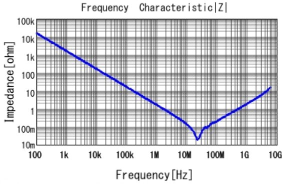
■ GRM188R72A104KA35 |Z| DCOV, 25degC
