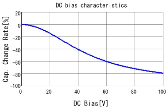
■ GRM188R72A104KA35 C-DC bias capchange, 25.0degC, AC1.
