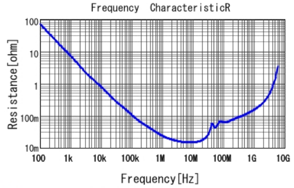
■ GRM188R72A104KA35 R DCOV, 25degC
