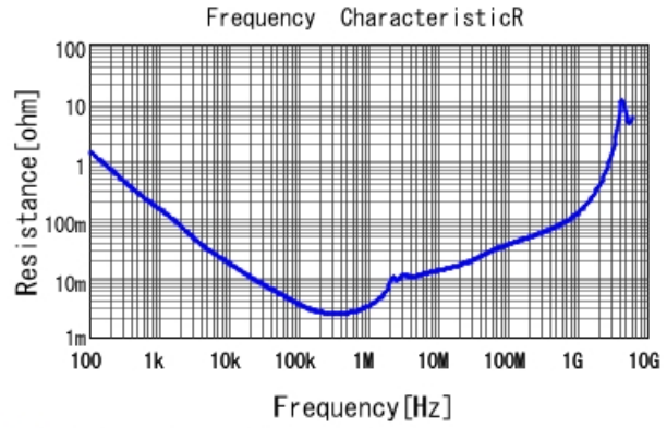
■ GRM31CC81E226KE11 R DCOV, 25degC
