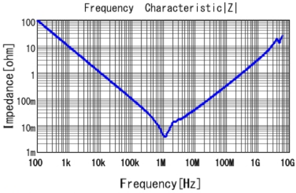
■ GRM31CC81E226KE11 |Z| DCOV, 25degC
