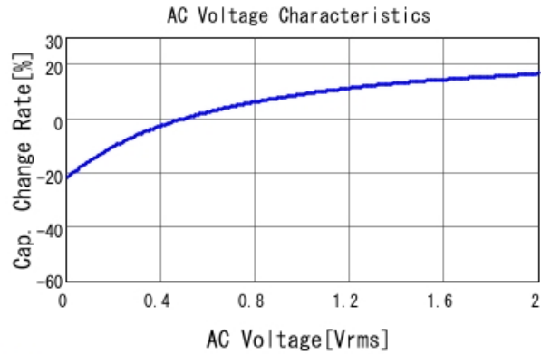
■ GRM31CC81E226KE11 C-AC Voltage capchange, DCOV, 25.0d
