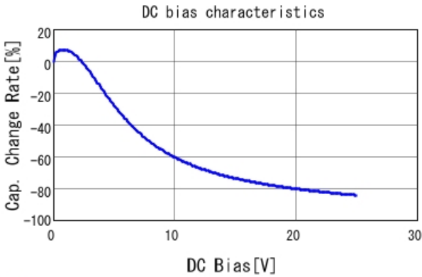
■ GRM31CC81E226KE11 C-DC bias capchange, 25.0degC, AC0.
