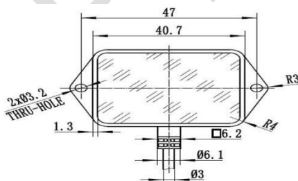
Figure 1. Front view of HPS-166S-L
