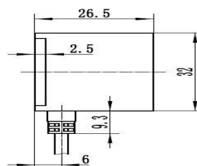
Figure 2. Side view of HPS-166S-L
