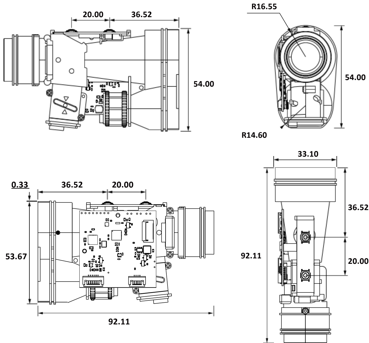
Picture 3-2 Module structure dimensions (unit: mm)
