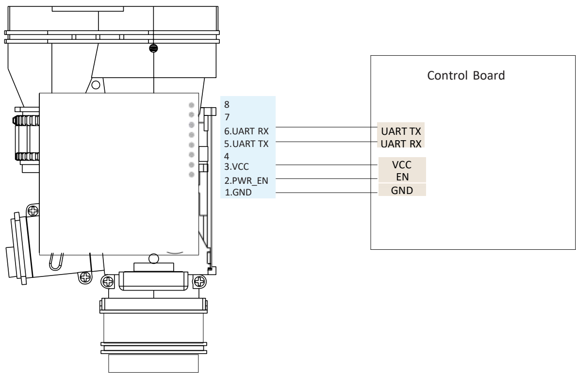
Picture 4-1 Module pin
