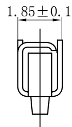
SECTION C-C
